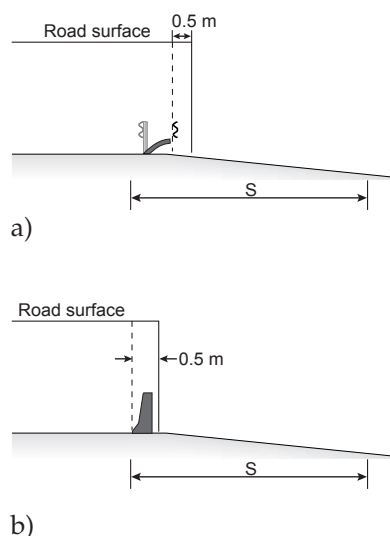
Figure 2.7 a) b) Overhead clearance in the safety zone at locations with safety barriers
