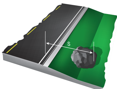
Figure 2.13 Example of a hazardous roadside obstacle which should not be found within the safety zone
