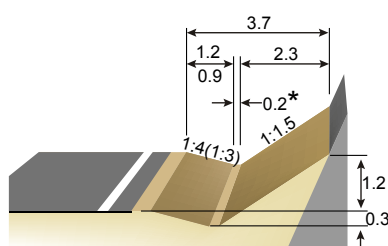
b) Side slope gradient of 1:1.5
