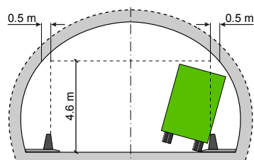
Figure 3.11 Overhead safety zone
