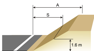
c) Gradient more than 1:2
