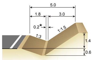
Figure 2.10 Requirements for open ditches (speed limit \leq 80\text{km/h} ).
