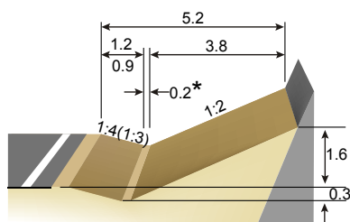
a) Side slope gradient of 1:2 .
