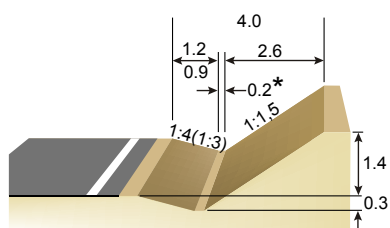
b) side slope 1:1.5
